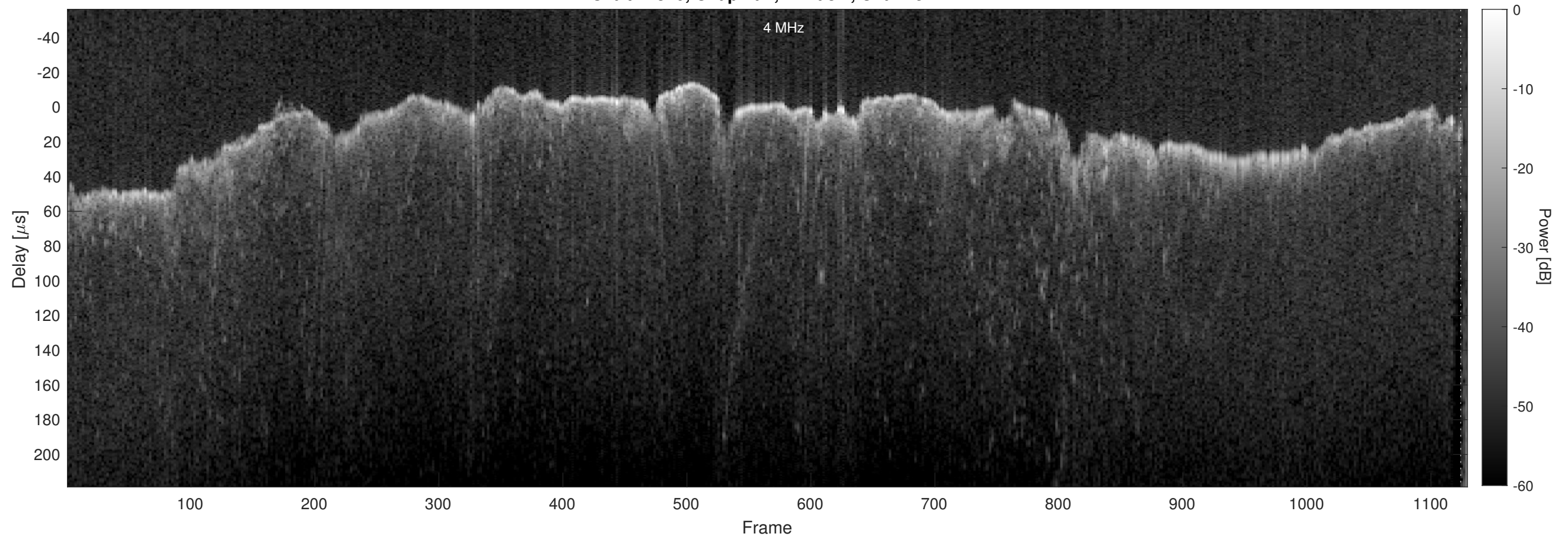
Orbit 12320, Chapman, Window, Channel 2
