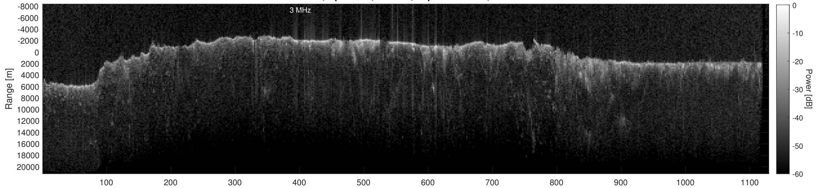
Orbit 12320, Depth-Corrected Cluttergram
