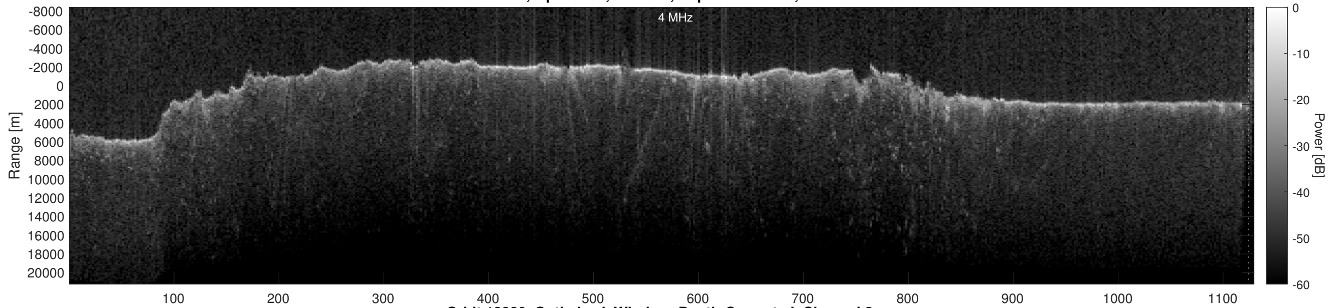
Orbit 12320, Optimized, Window, Depth-Corrected, Channel 2
