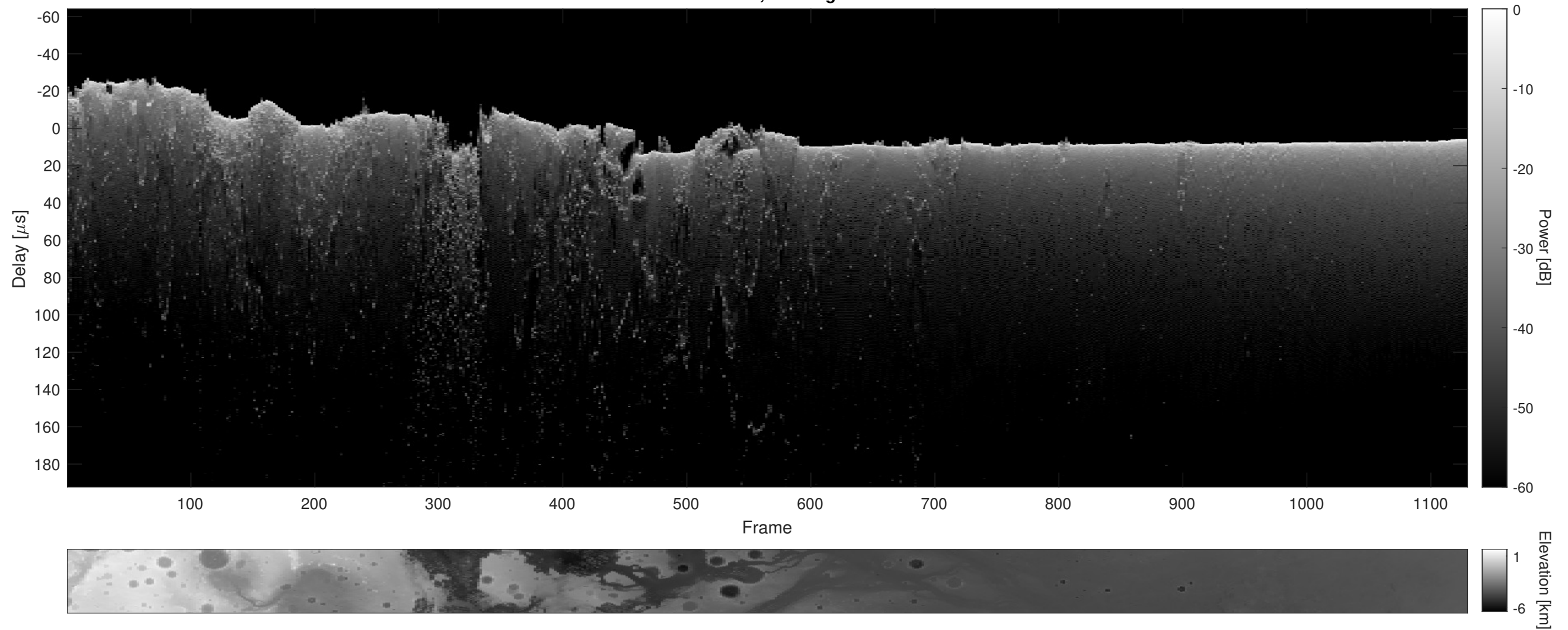
Orbit 12321, Cluttergram
