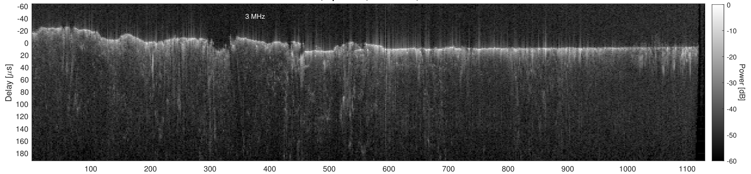
Orbit 12321, Cluttergram
