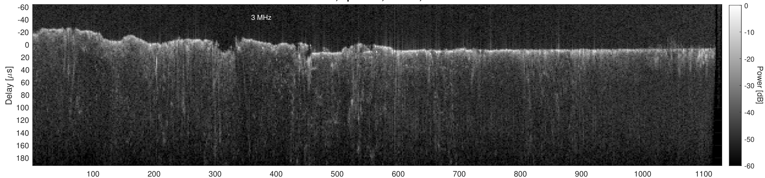
Orbit 12321, Cluttergram
