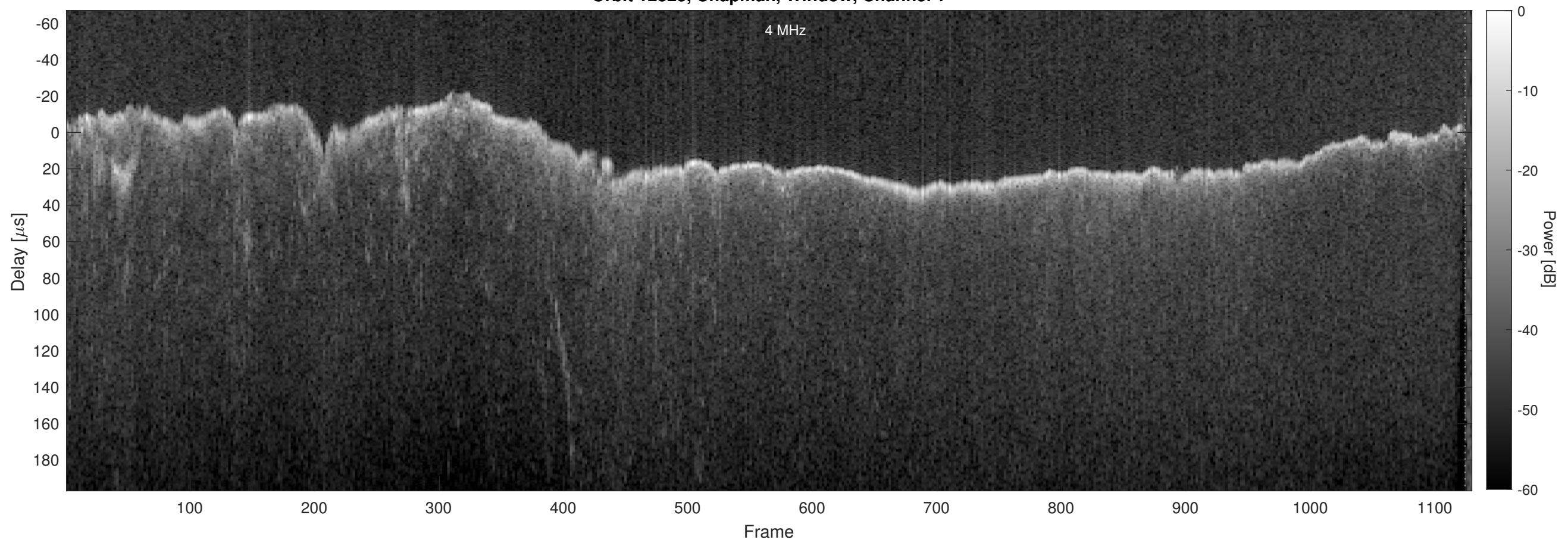
Orbit 12323, Chapman, Window, Channel 2
