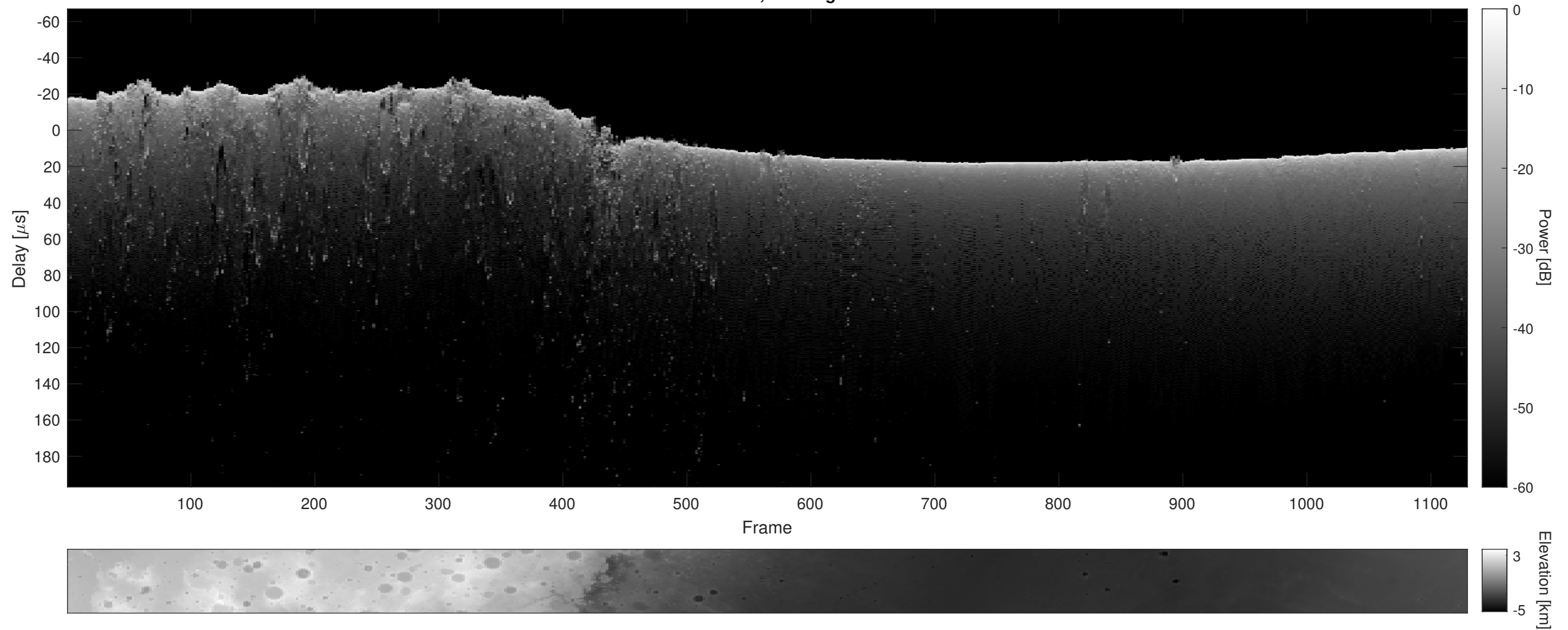
Orbit 12323, Cluttergram
