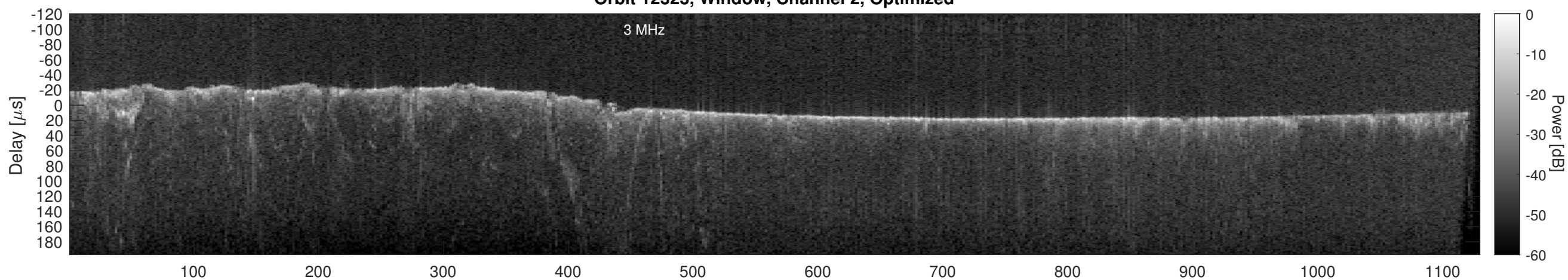
Orbit 12323, Cluttergram
