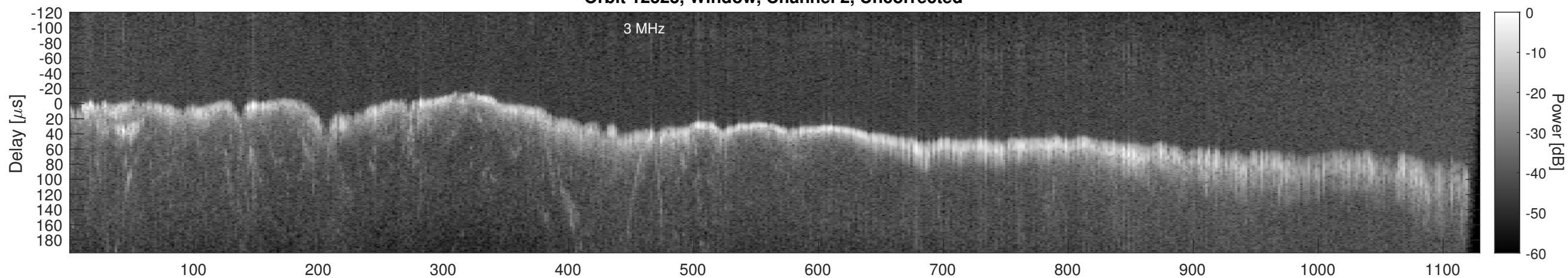
Orbit 12323, Window, Channel 2, Chapman
