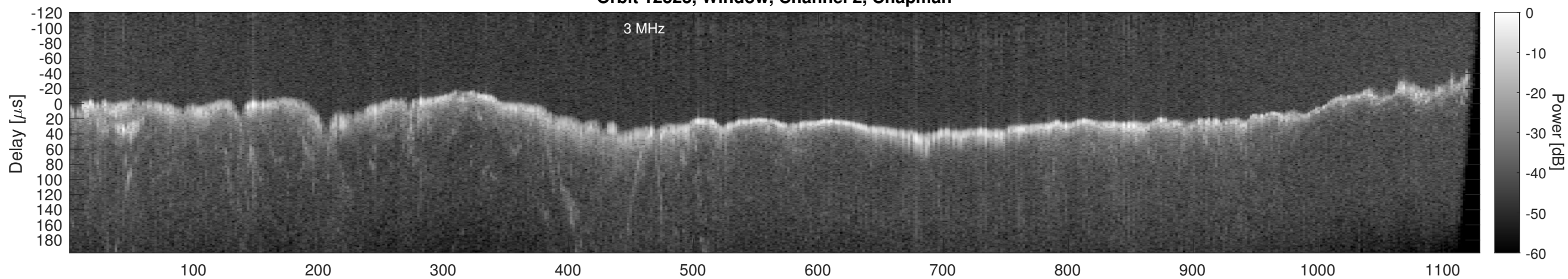
Orbit 12323, Window, Channel 2, Optimized
