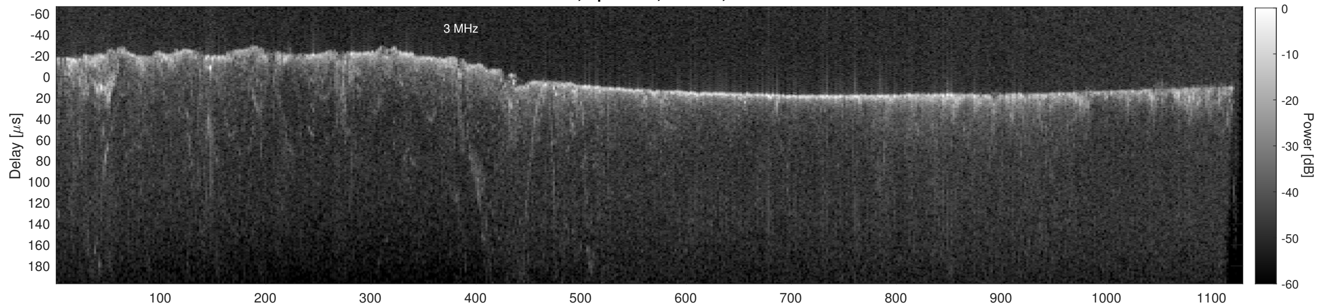
Orbit 12323, Cluttergram
