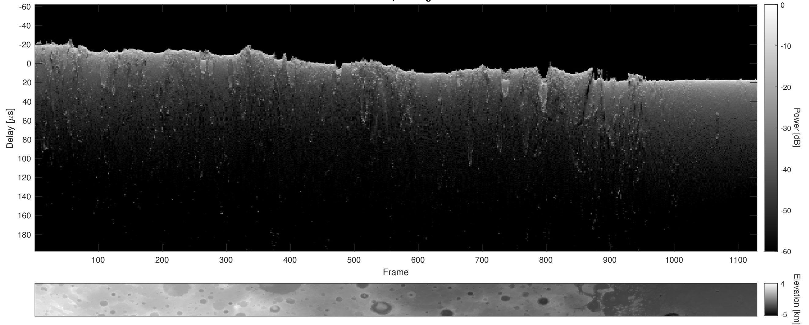
Orbit 12324, Cluttergram
