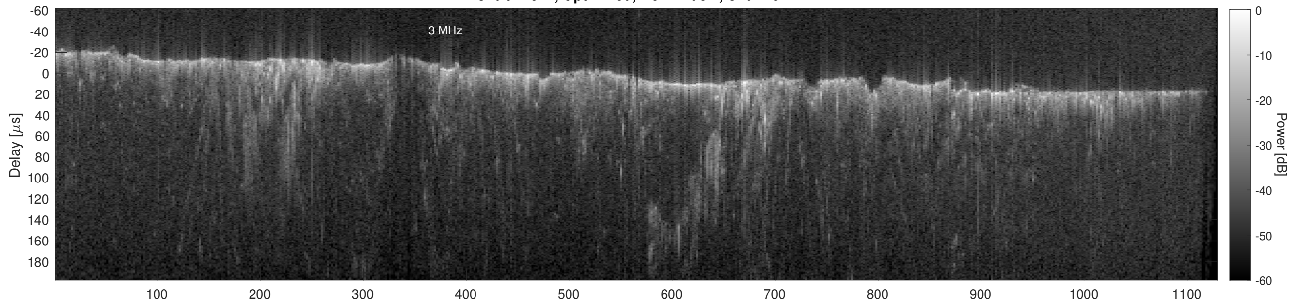
Orbit 12324, Cluttergram
