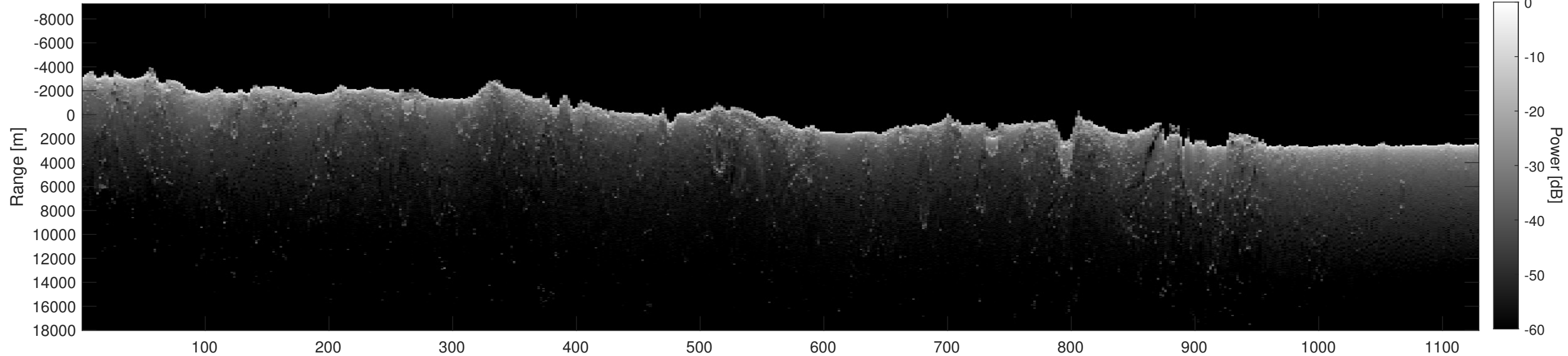
Orbit 12324, Depth-Corrected Cluttergram
