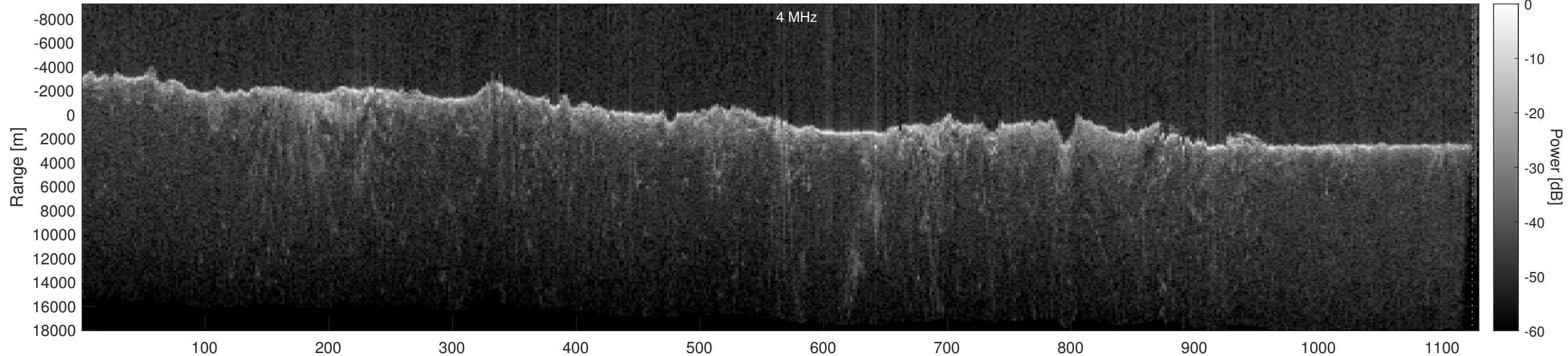
Orbit 12324, Optimized, Window, Depth-Corrected, Channel 2
