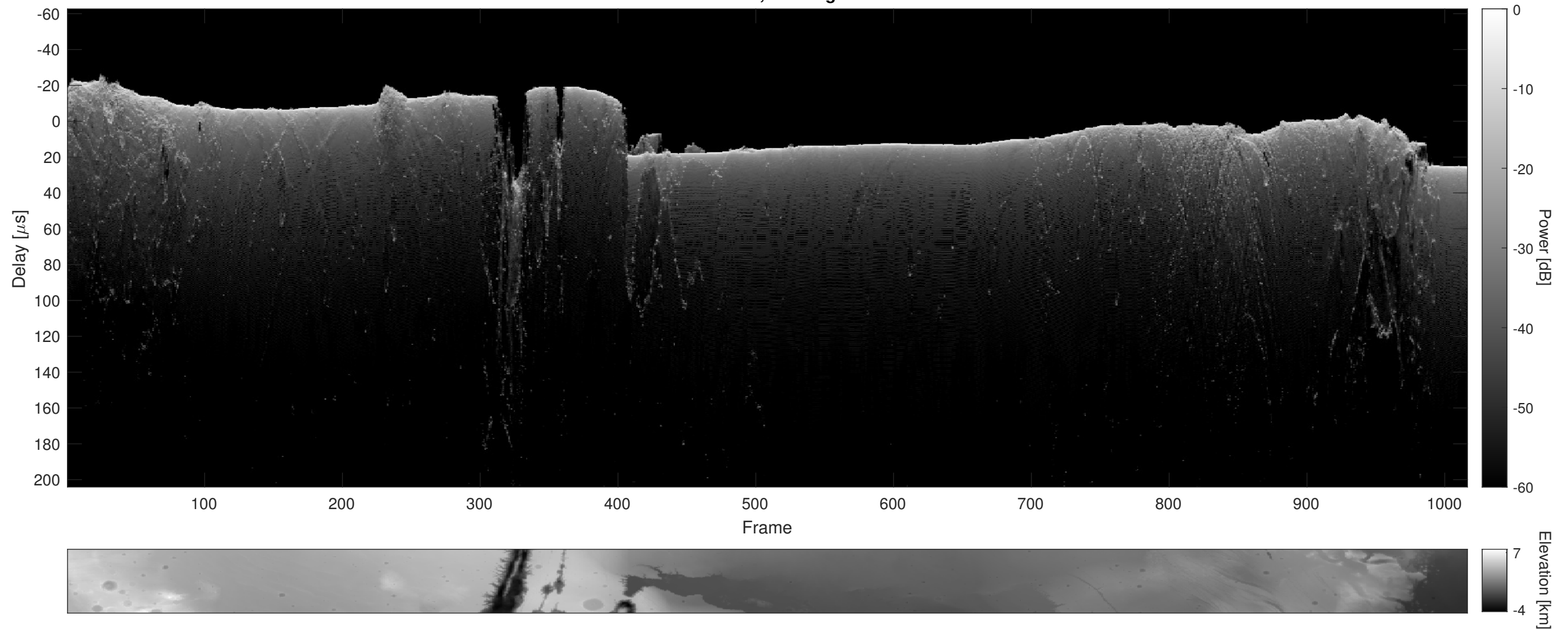
Orbit 12325, Cluttergram
