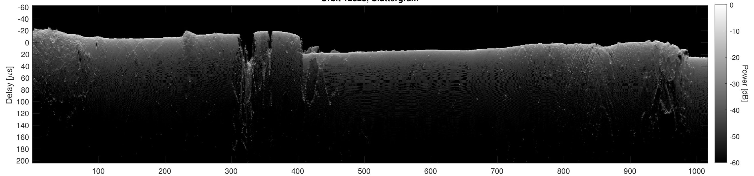
Orbit 12325, Cluttergram
