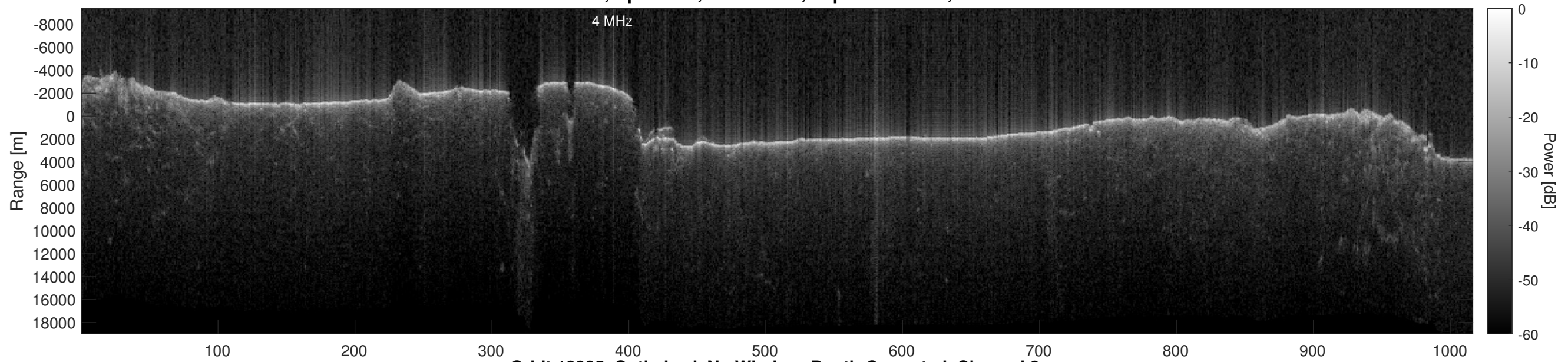
Orbit 12325, Optimized, No Window, Depth-Corrected, Channel 2
