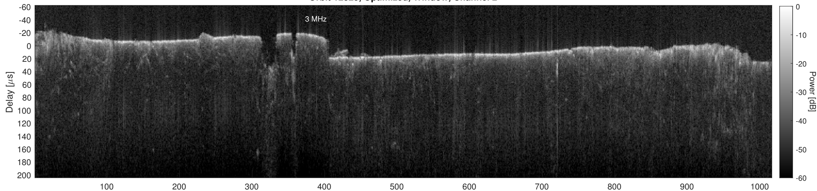
Orbit 12325, Cluttergram
