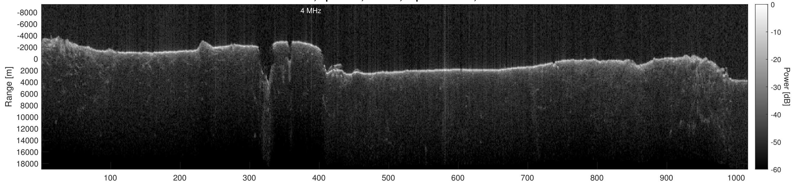
Orbit 12325, Optimized, Window, Depth-Corrected, Channel 2
