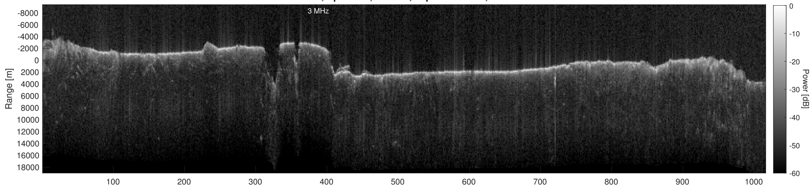
Orbit 12325, Depth-Corrected Cluttergram
