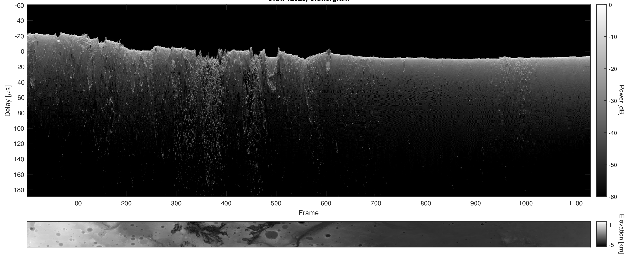
Orbit 12328, Cluttergram
