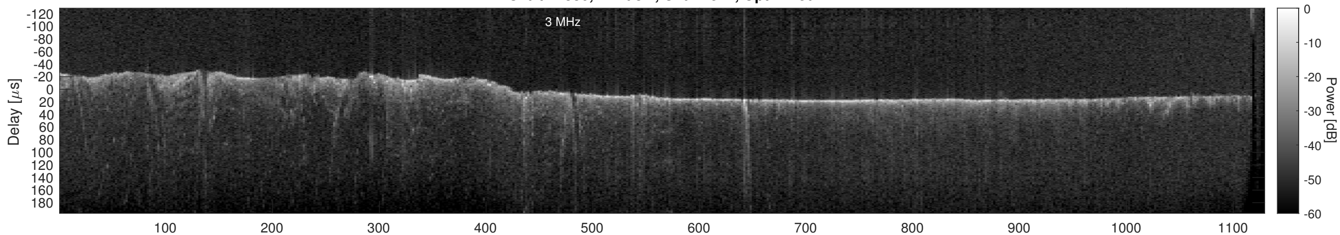
Orbit 12330, Cluttergram
