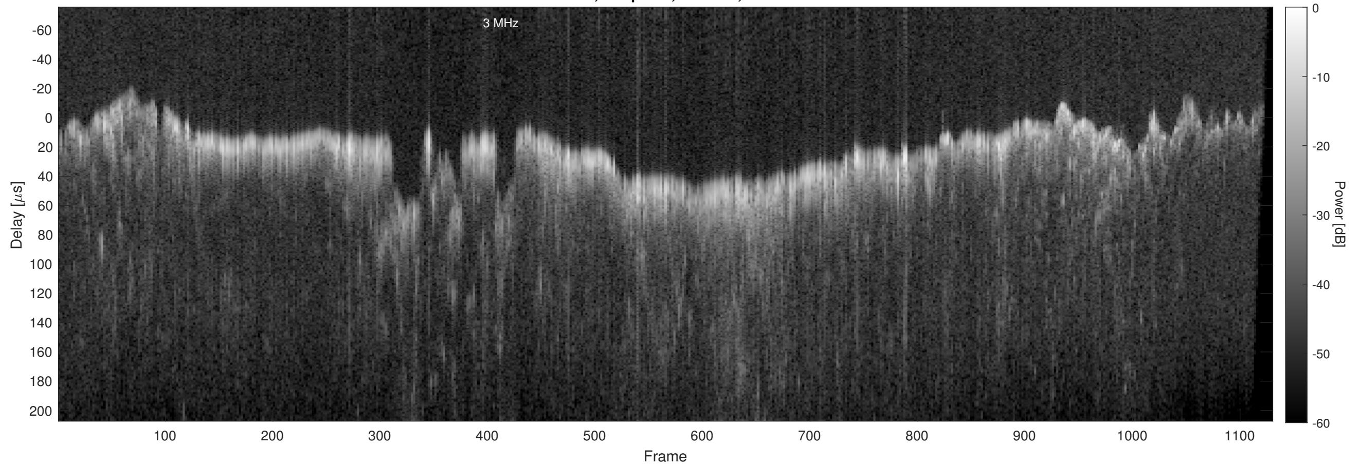
Orbit 12332, Chapman, Window, Channel 2
