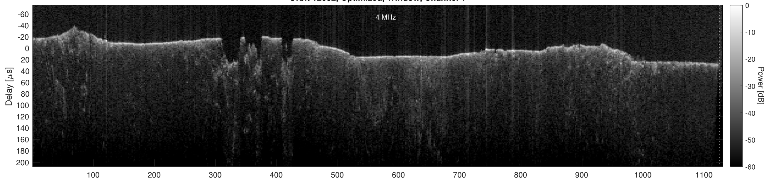
Orbit 12332, Optimized, Window, Channel 2
