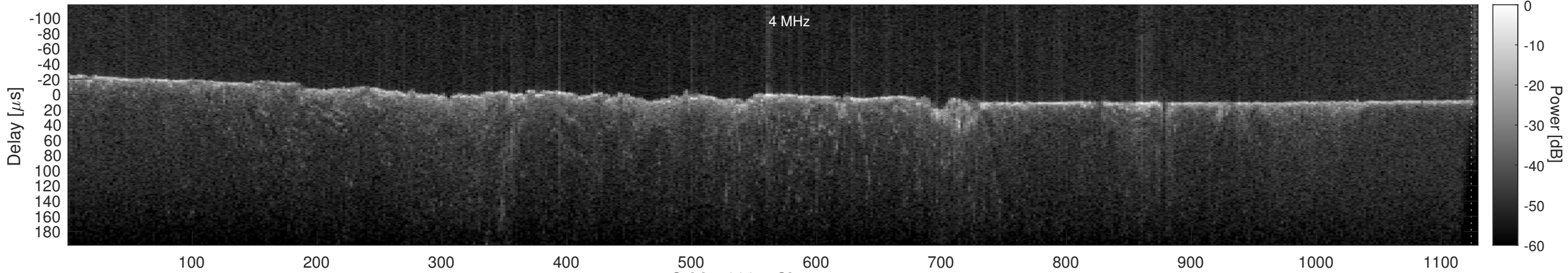
Orbit 12335, Cluttergram
