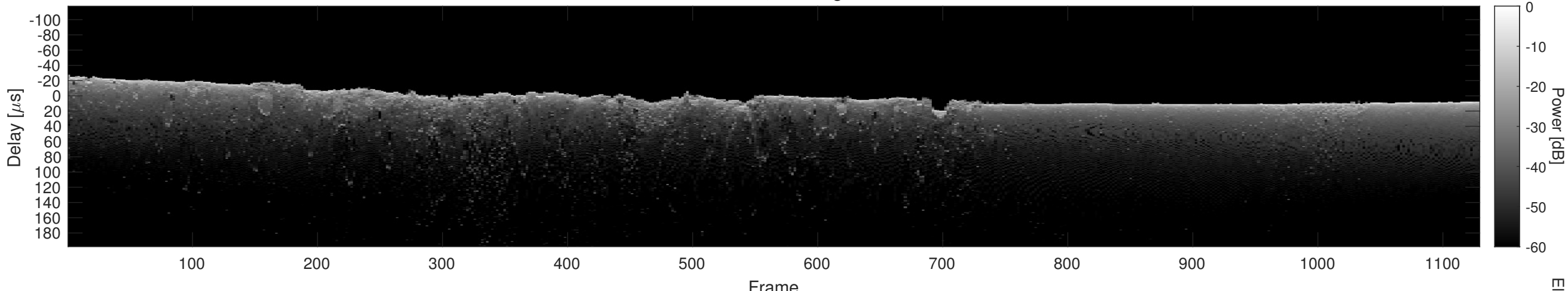
Orbit 12335, Cluttergram
