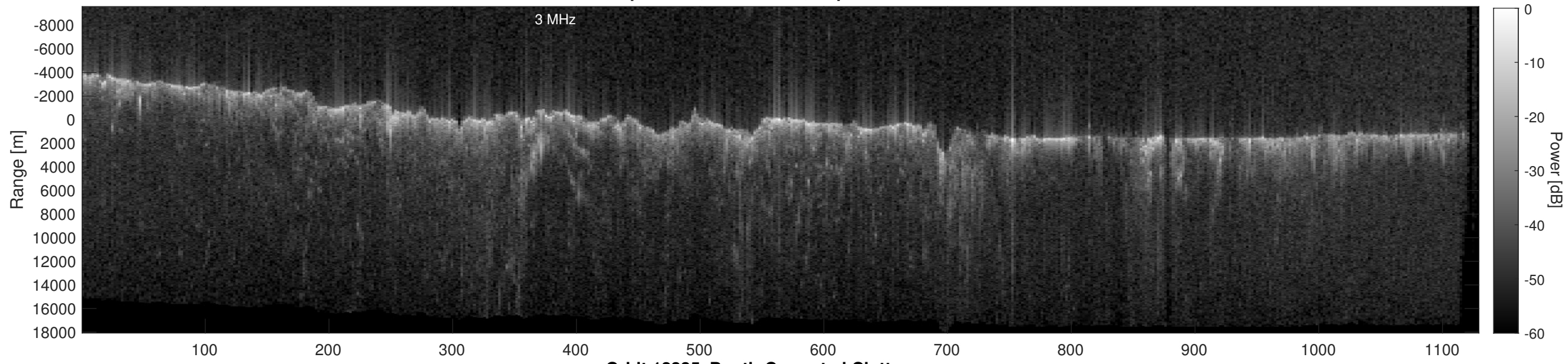
Orbit 12335, Depth-Corrected Cluttergram
