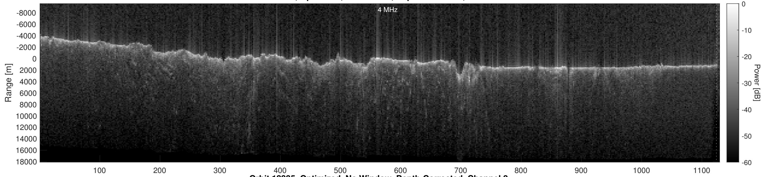
Orbit 12335, Optimized, No Window, Depth-Corrected, Channel 2
