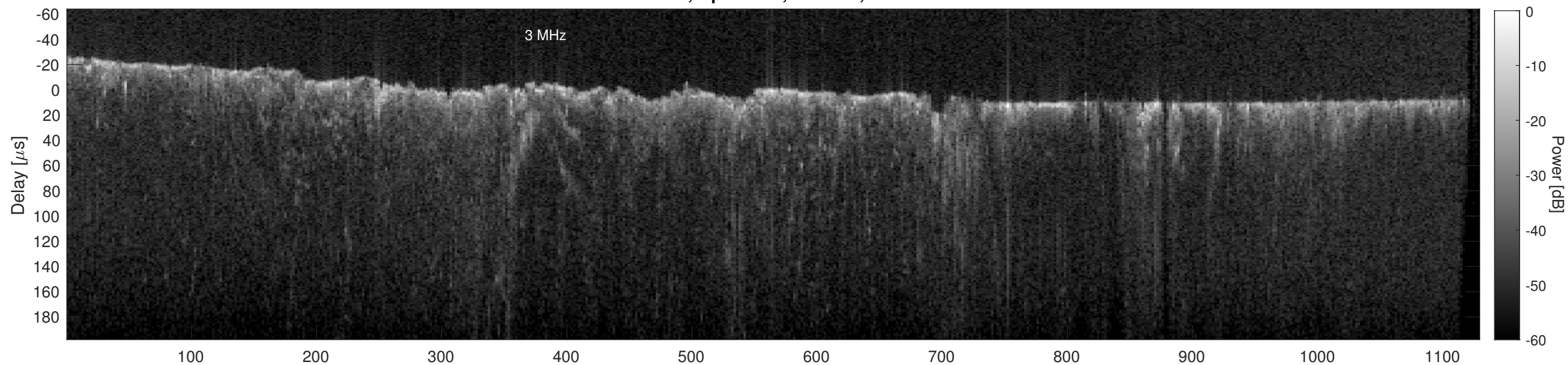
Orbit 12335, Cluttergram
