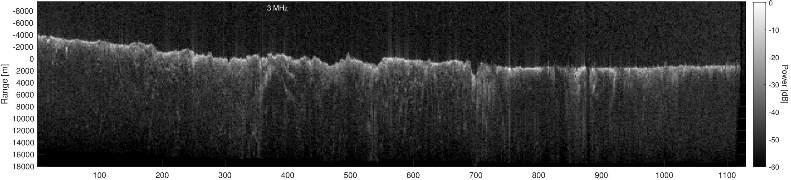
Orbit 12335, Depth-Corrected Cluttergram
