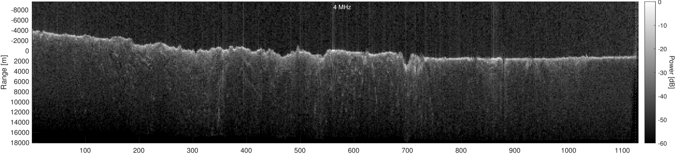
Orbit 12335, Optimized, Window, Depth-Corrected, Channel 2
