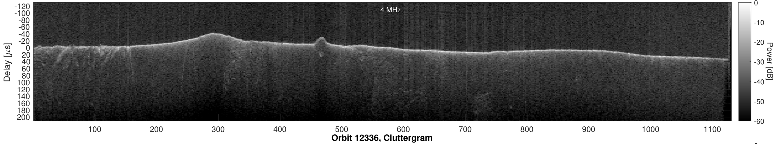
Orbit 12336, Window, Channel 1, Optimized
