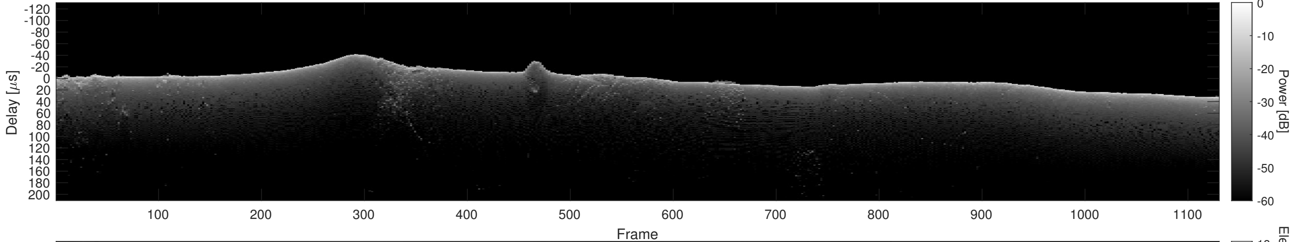
Orbit 12336, Cluttergram
