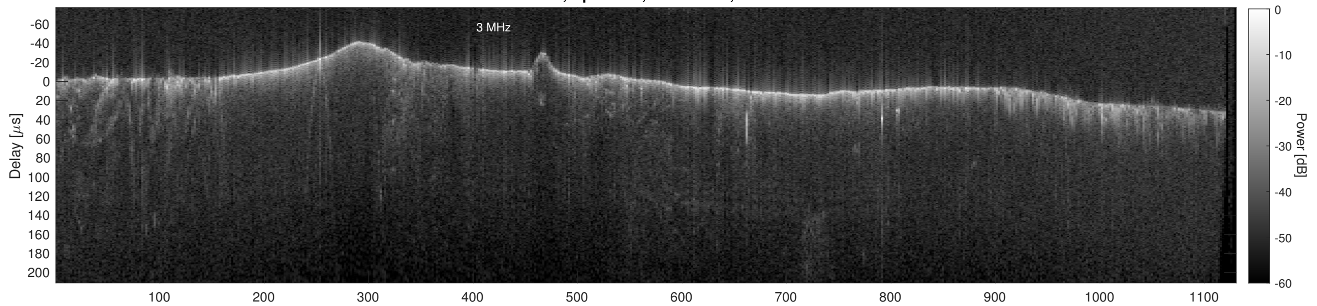
Orbit 12336, Cluttergram
