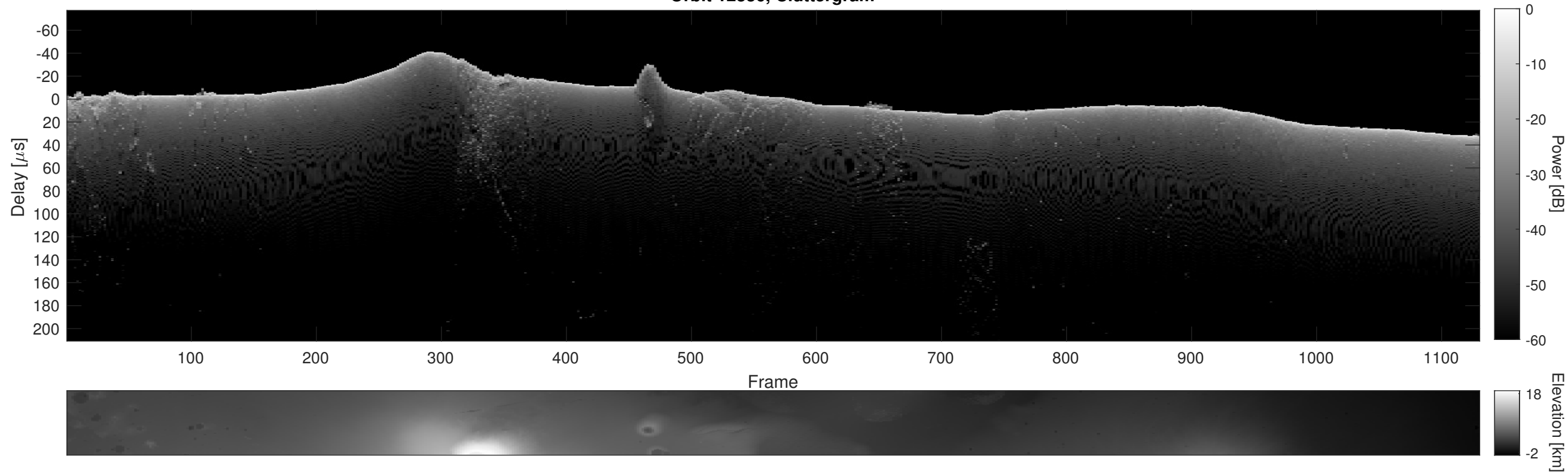
Orbit 12336, Cluttergram
