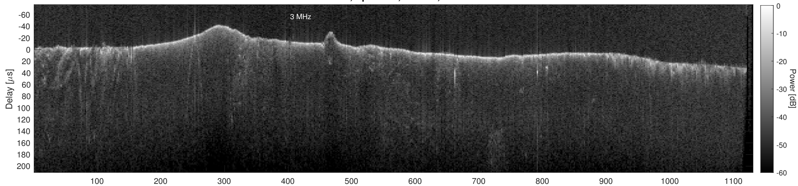
Orbit 12336, Cluttergram
