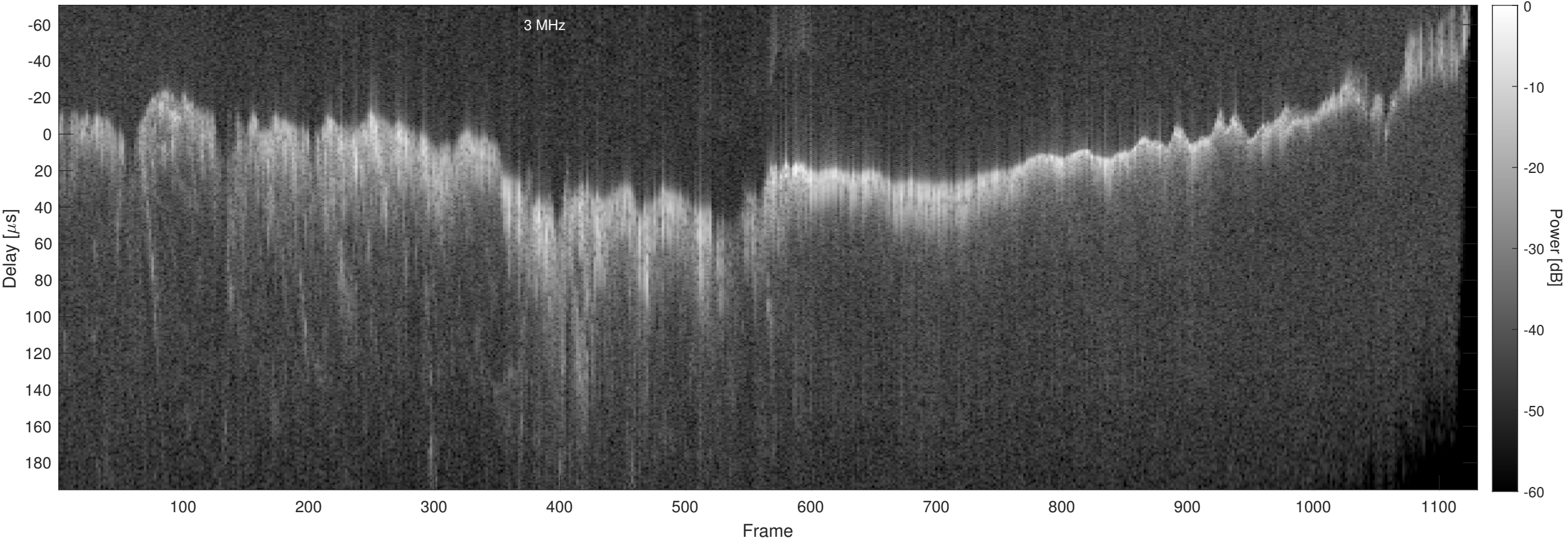
Orbit 12337, Chapman, No Window, Channel 2
