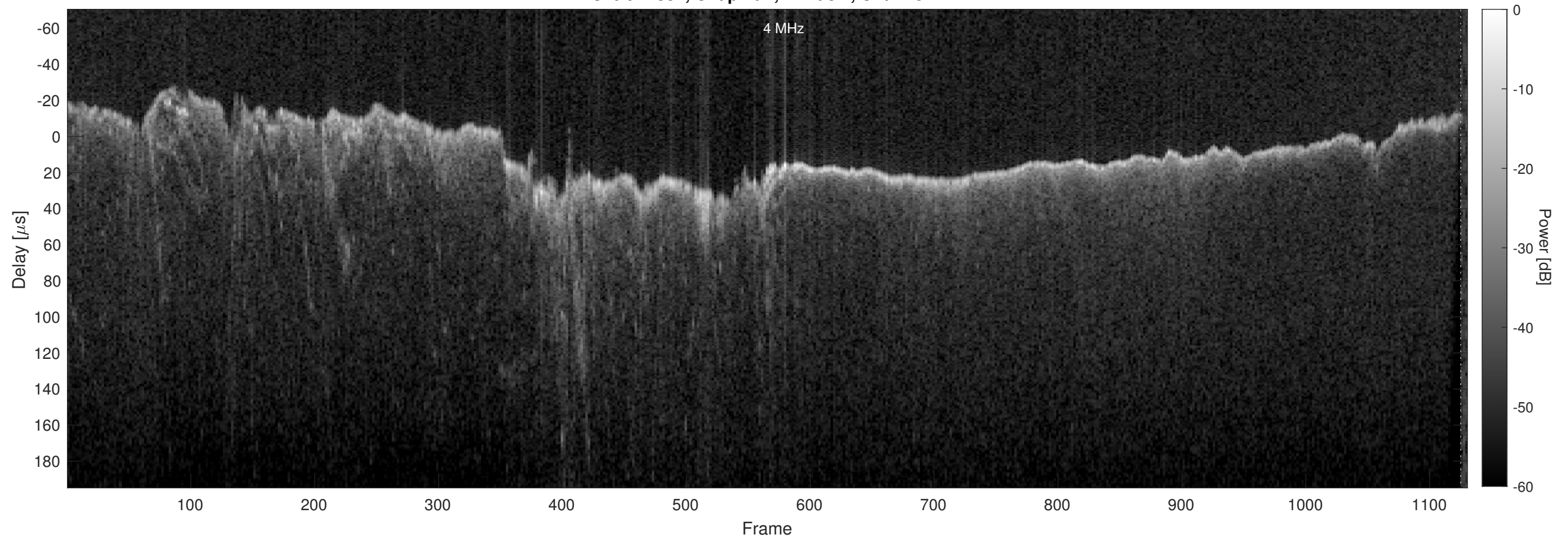
Orbit 12337, Chapman, Window, Channel 2
