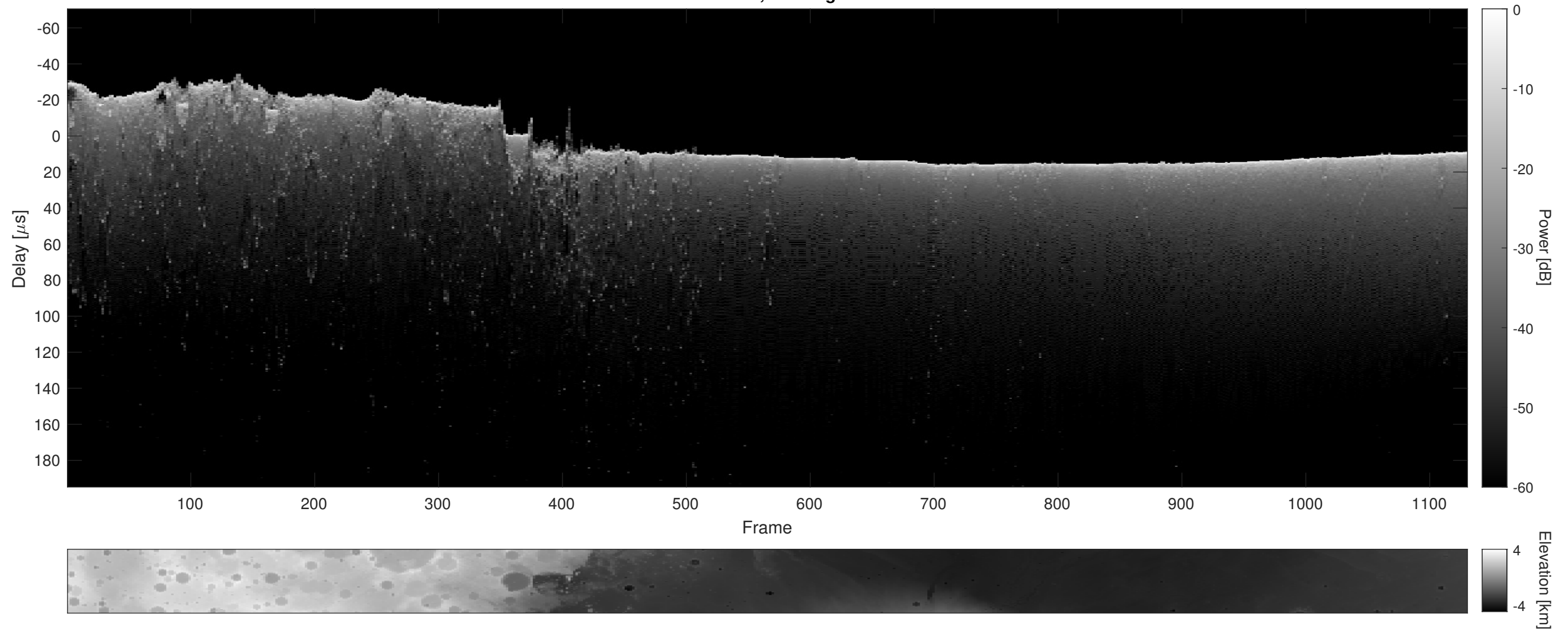
Orbit 12337, Cluttergram
