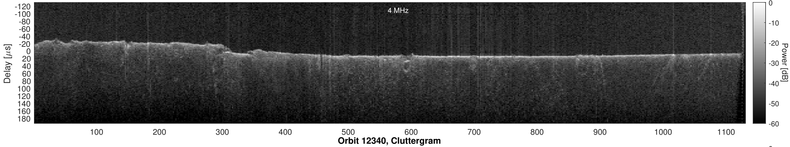
Orbit 12340, Window, Channel 1, Optimized
