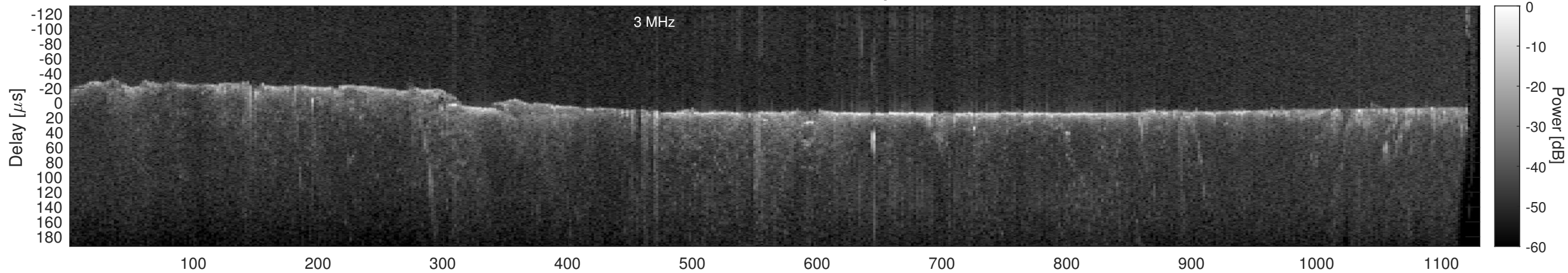
Orbit 12340, Cluttergram
