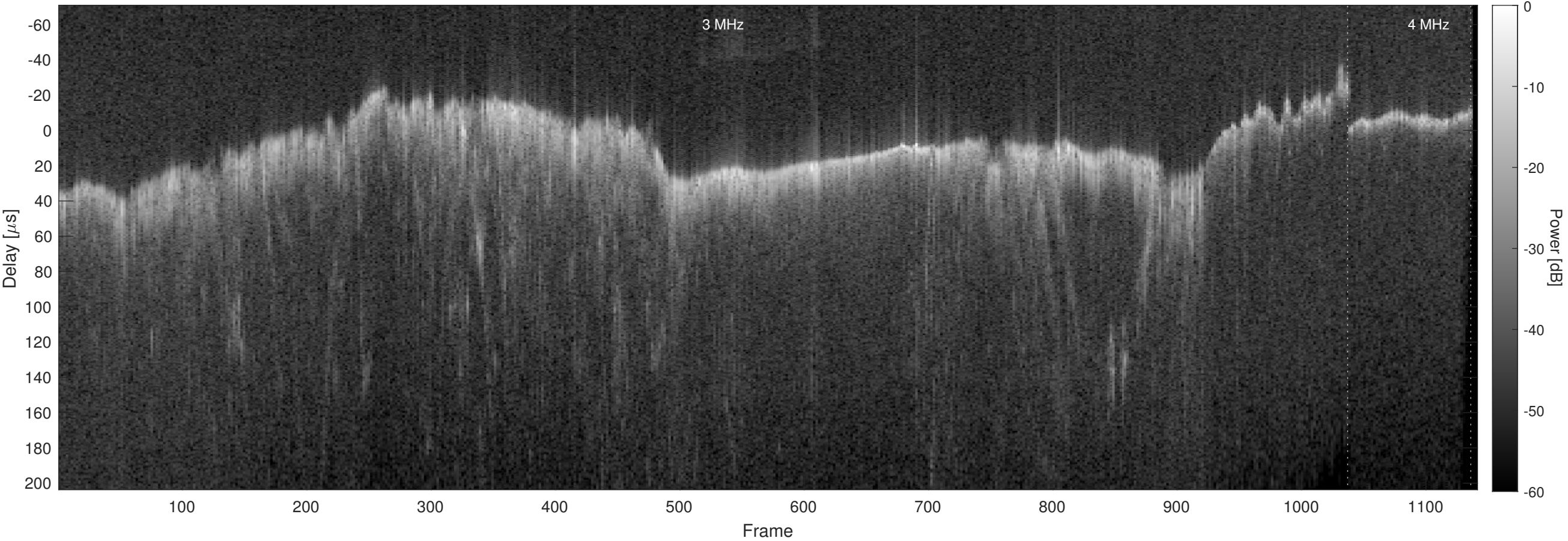
Orbit 12341, Chapman, No Window, Channel 2
