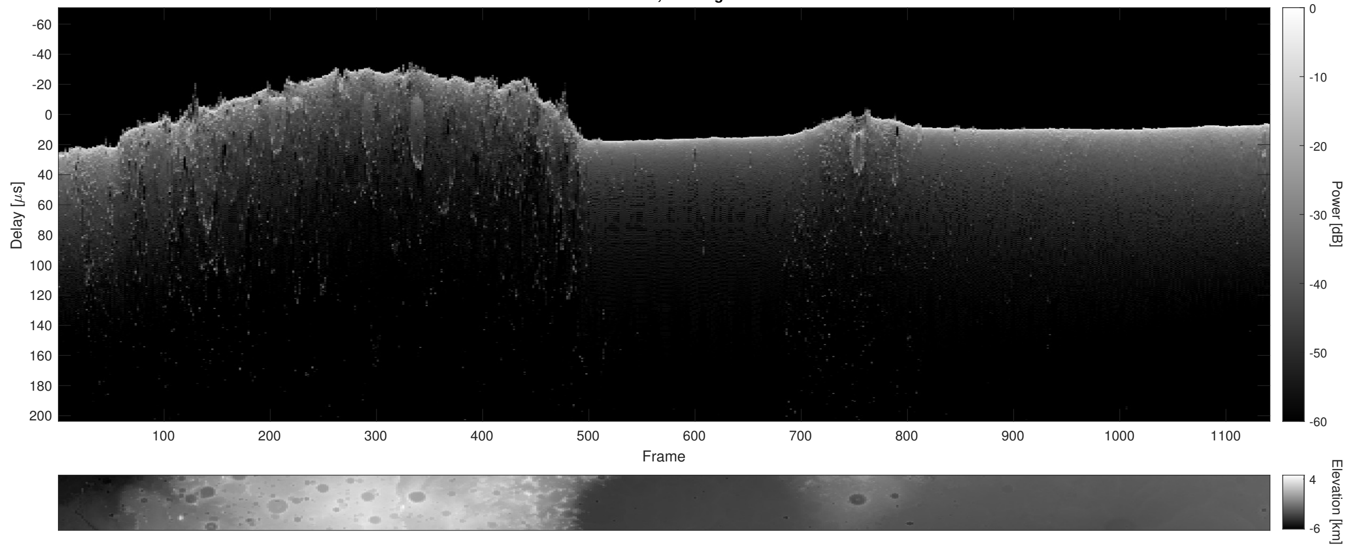
Orbit 12341, Cluttergram
