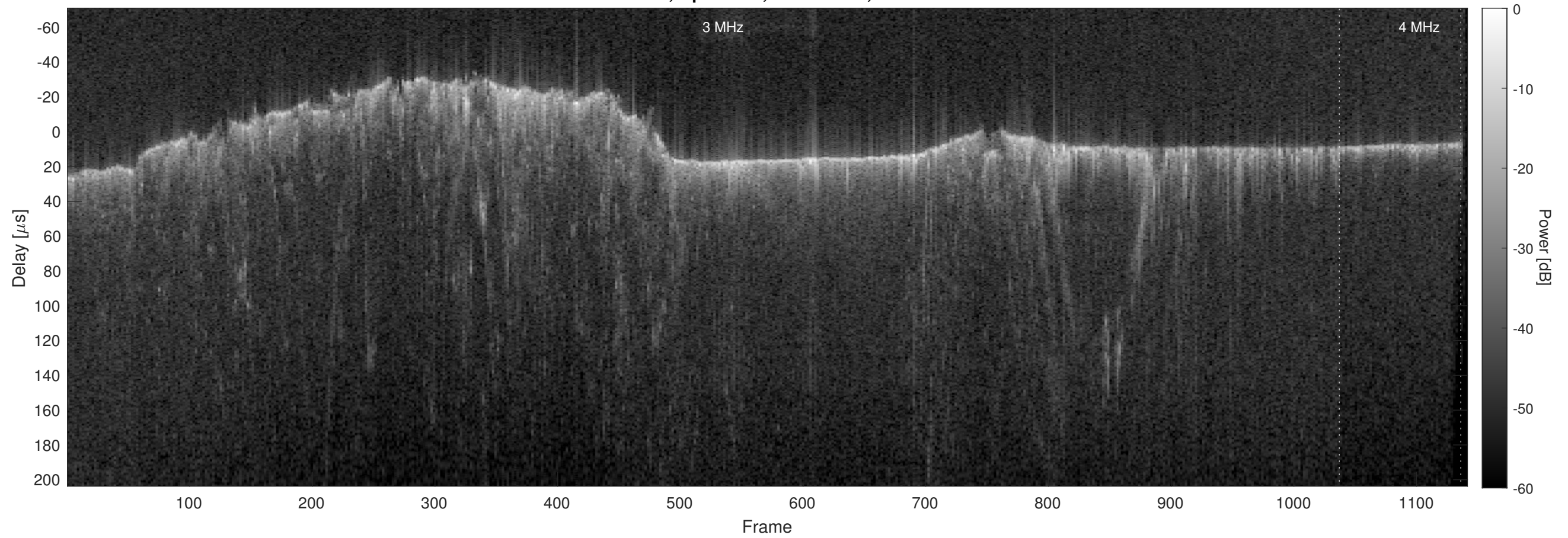
Orbit 12341, Optimized, No Window, Channel 2
