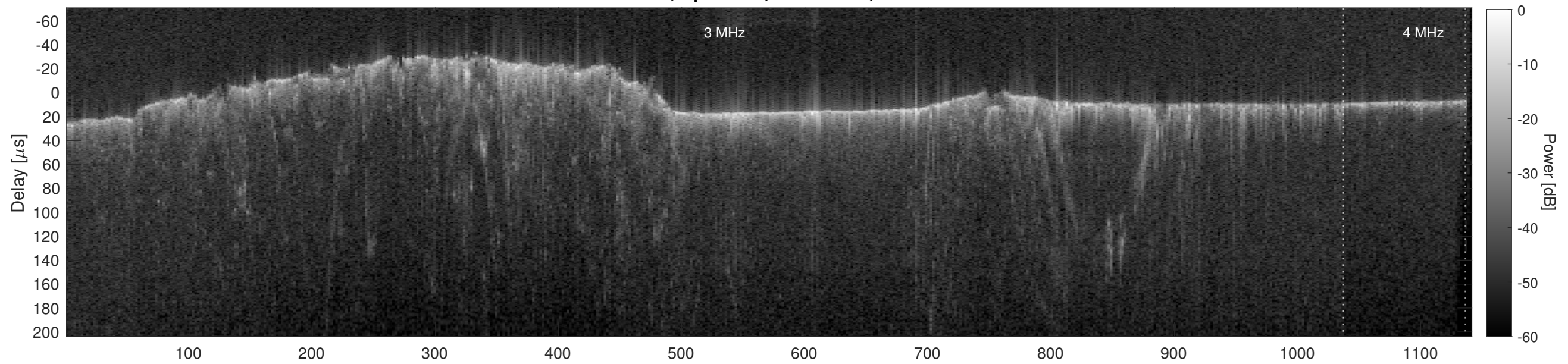
Orbit 12341, Cluttergram
