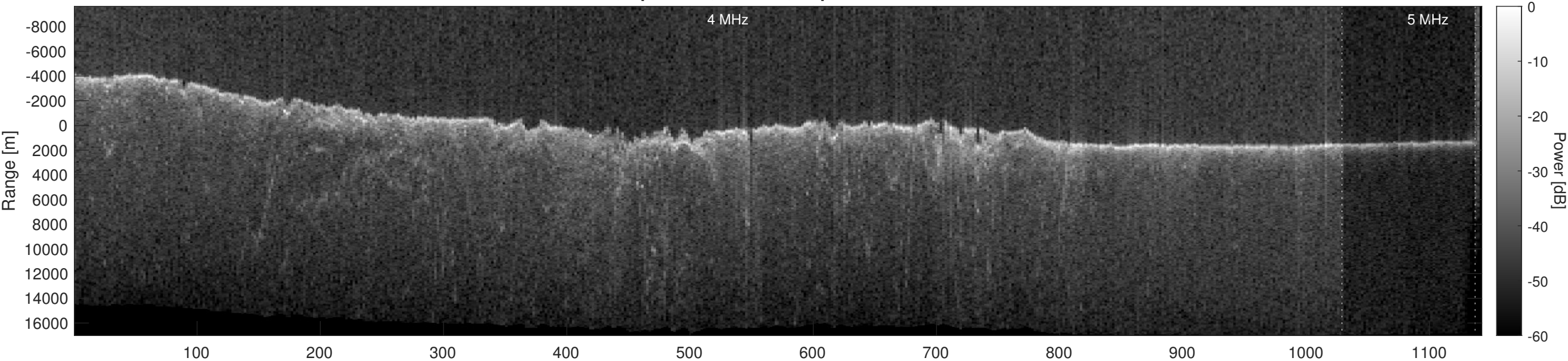
Orbit 12342, Optimized, Window, Depth-Corrected, Channel 2
