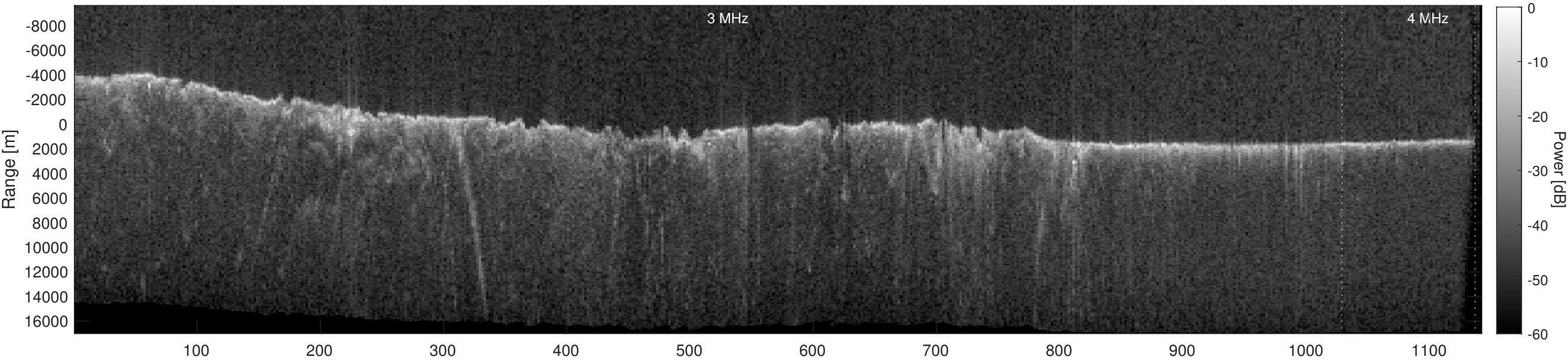
Orbit 12342, Depth-Corrected Cluttergram
