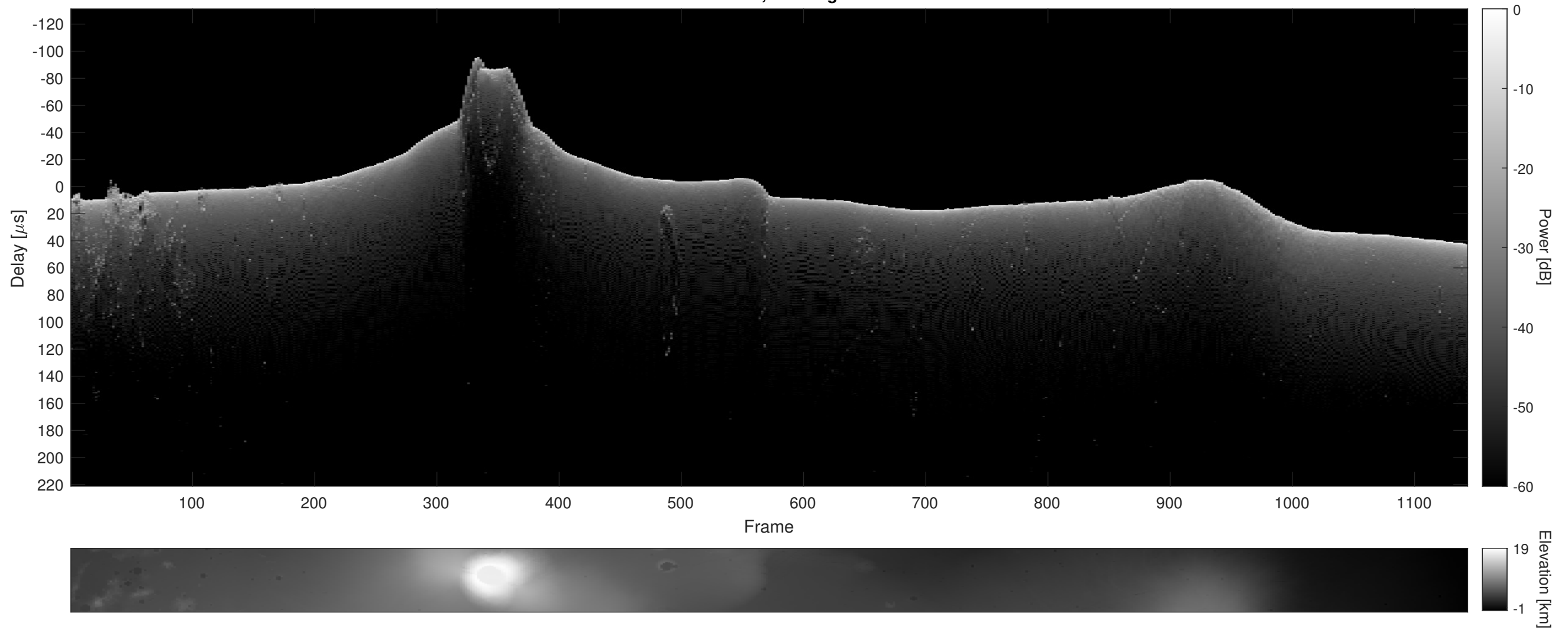
Orbit 12343, Cluttergram
