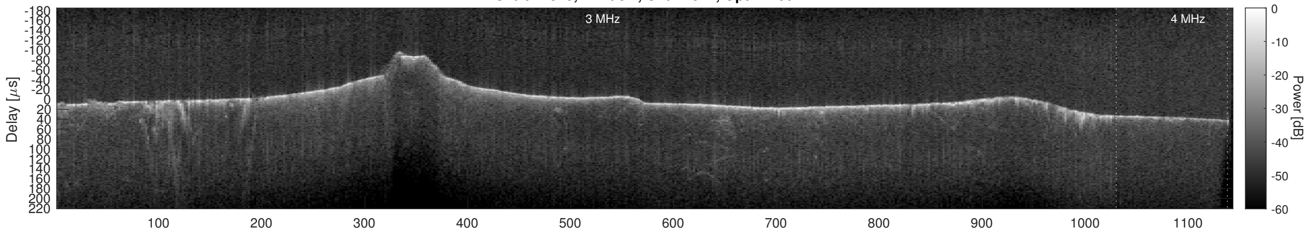
Orbit 12343, Cluttergram
