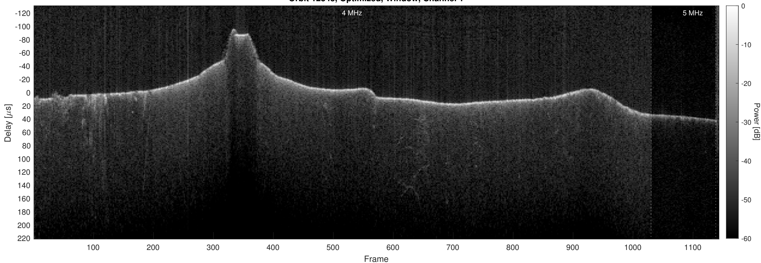
Orbit 12343, Optimized, Window, Channel 2
