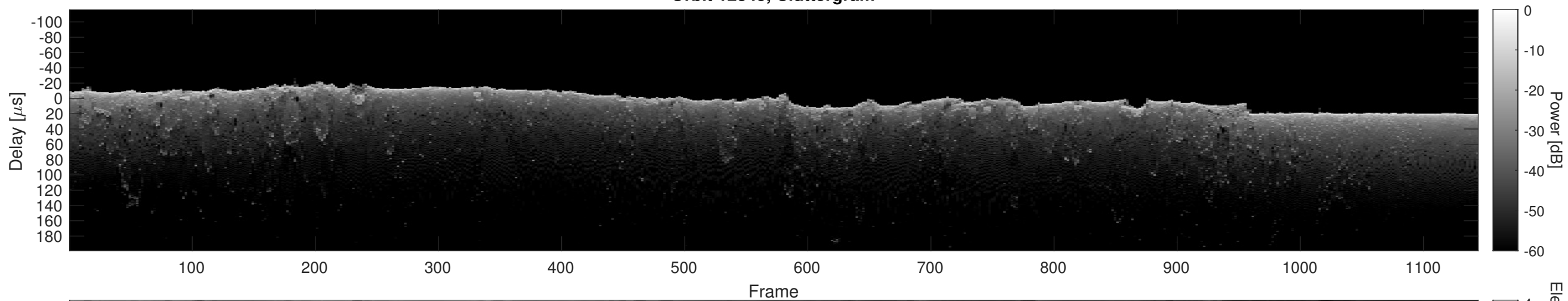
Orbit 12345, Cluttergram
