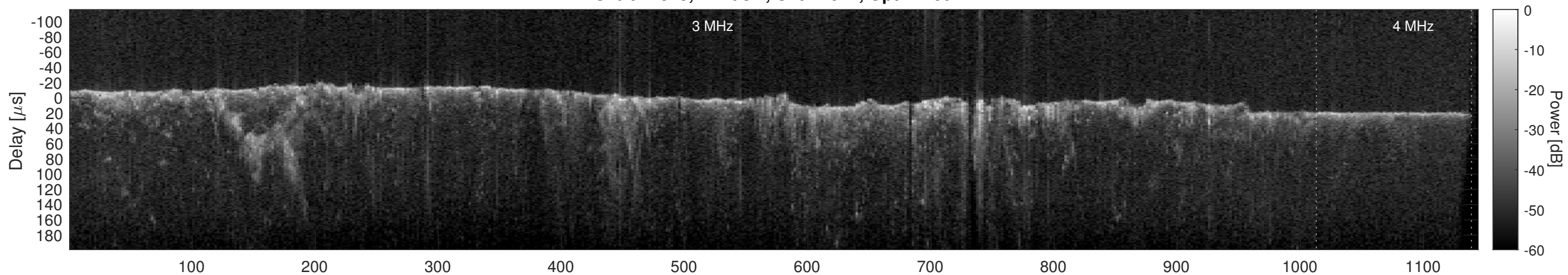
Orbit 12345, Cluttergram
