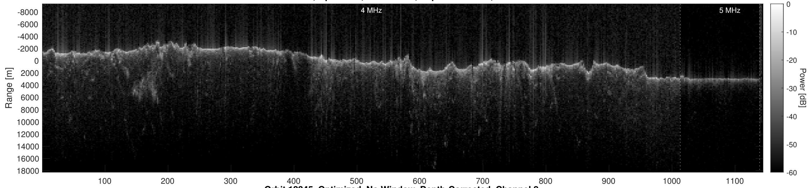
Orbit 12345, Optimized, No Window, Depth-Corrected, Channel 2
