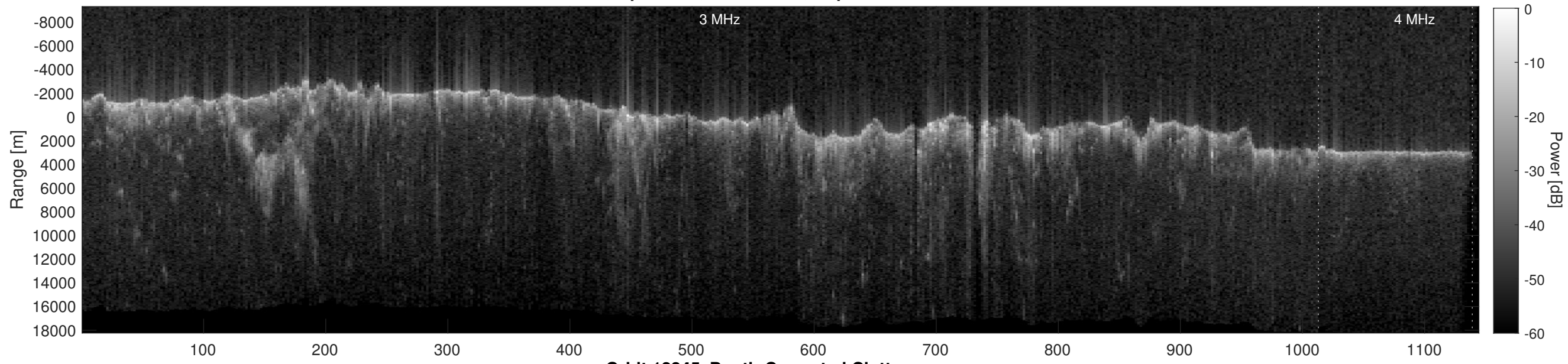
Orbit 12345, Depth-Corrected Cluttergram
