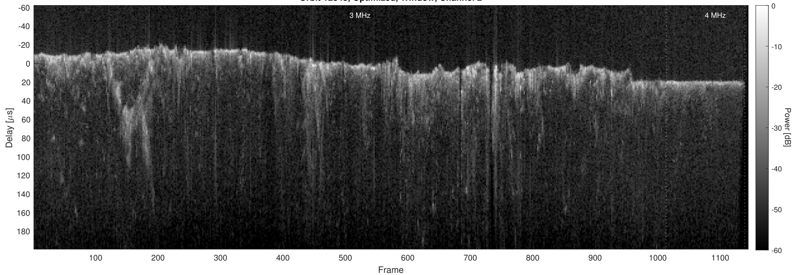
Orbit 12345, Optimized, Window, Channel 2
