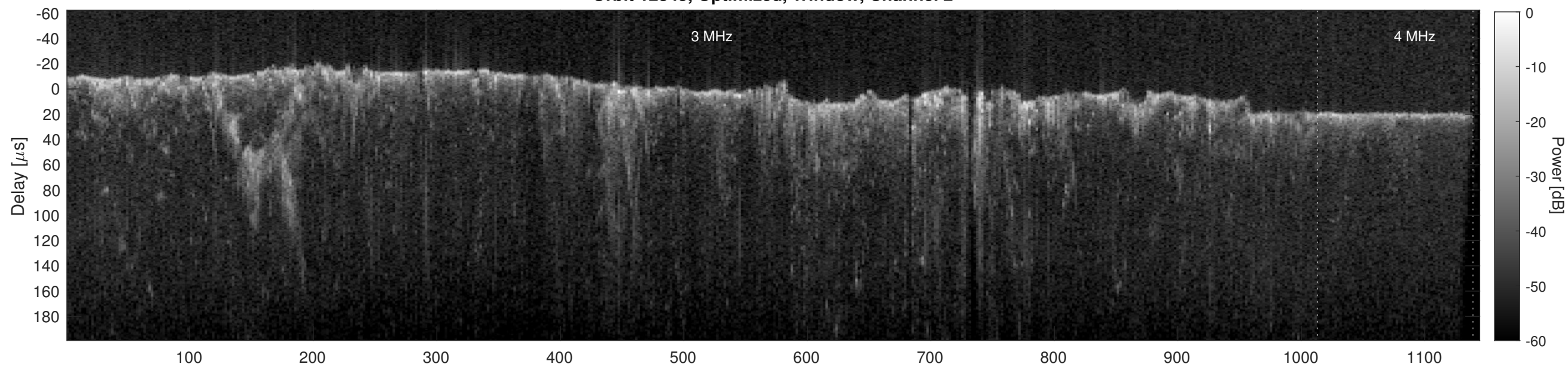
Orbit 12345, Cluttergram
