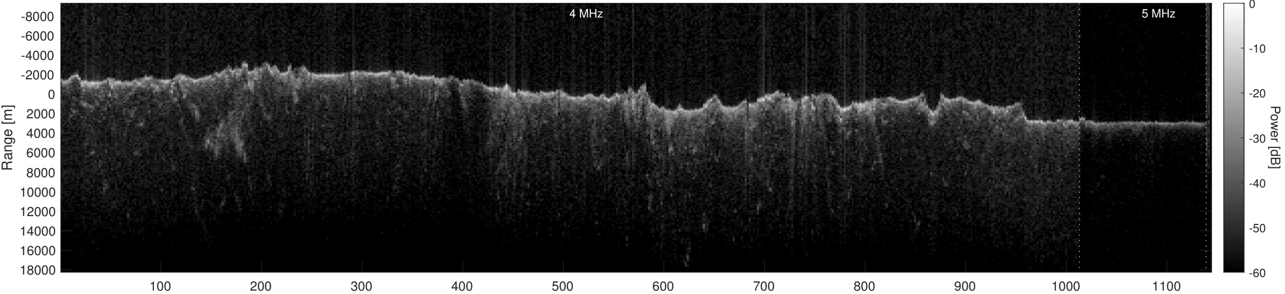
Orbit 12345, Optimized, Window, Depth-Corrected, Channel 2
