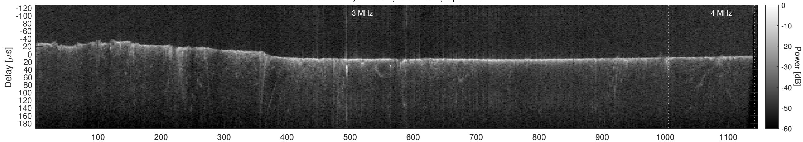
Orbit 12347, Cluttergram
