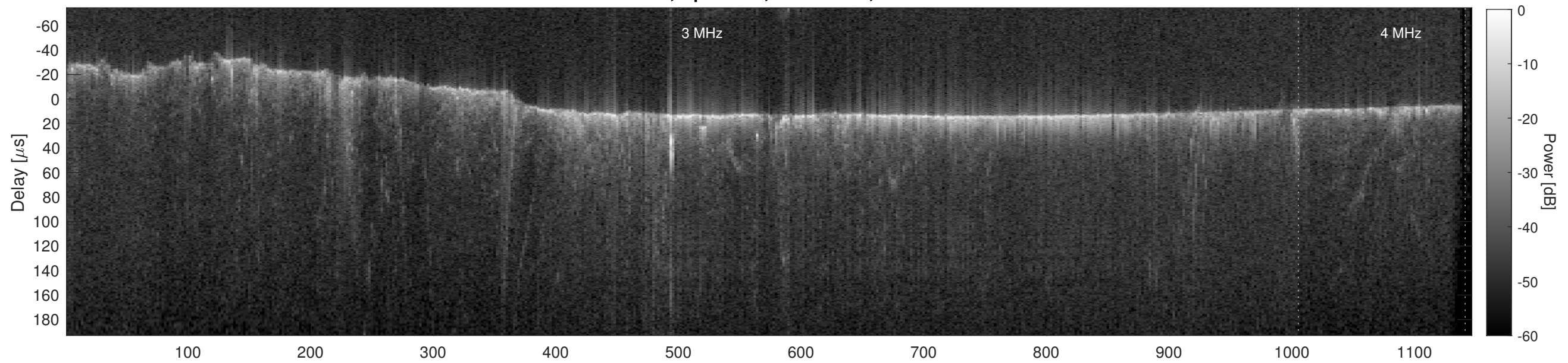
Orbit 12347, Cluttergram
