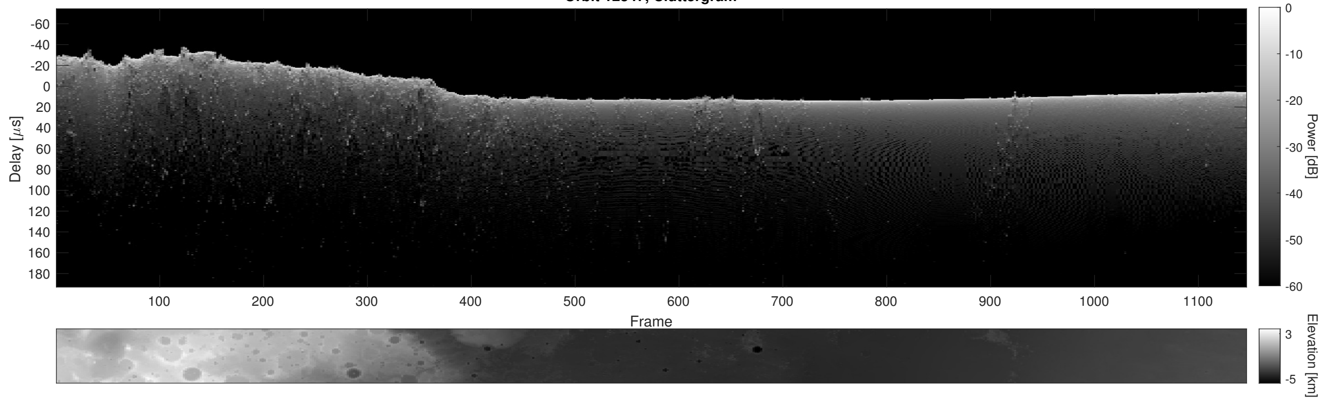
Orbit 12347, Cluttergram
