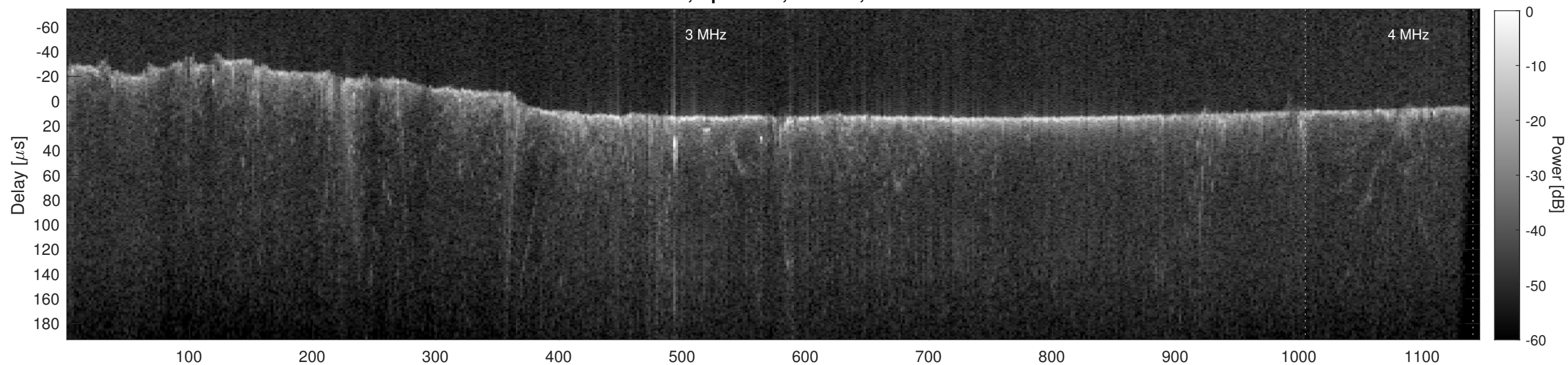
Orbit 12347, Cluttergram
